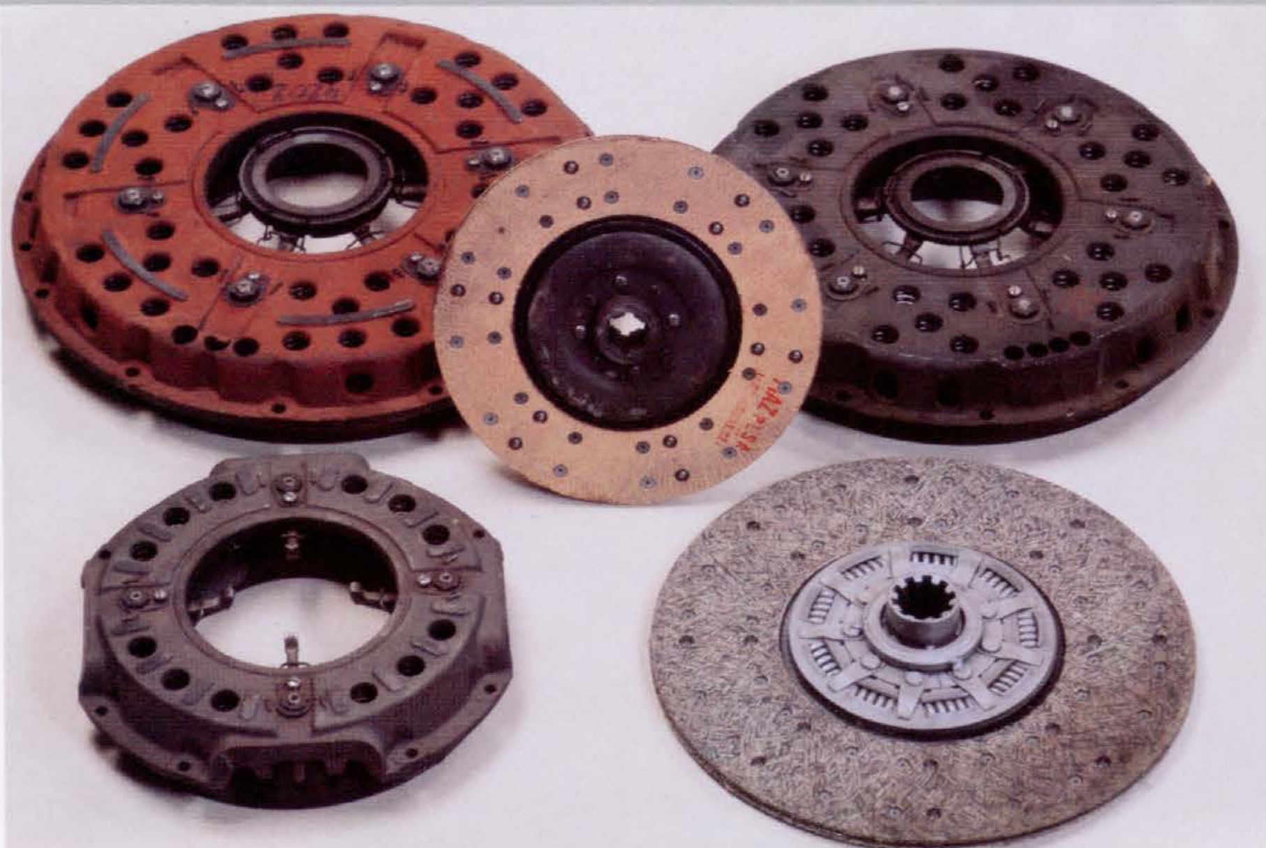
Single-plate, dry-disc CLUTCHES Diameter up to 475 mm Max. Torque up to 1150 Nm Manufacturer: RUEN Kočani FAMOS — Fabrika spojnice, Sanski most
