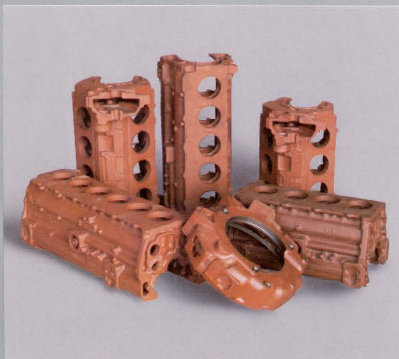
CASTINGS made of GREY- and NODULAR IRON for Motor Industry (Crankcases, Clutches, Gearboxes, Gearings, Flywheels, Brake Drums, etc.) partly machined Manufacturer: BELT Črnomelj
