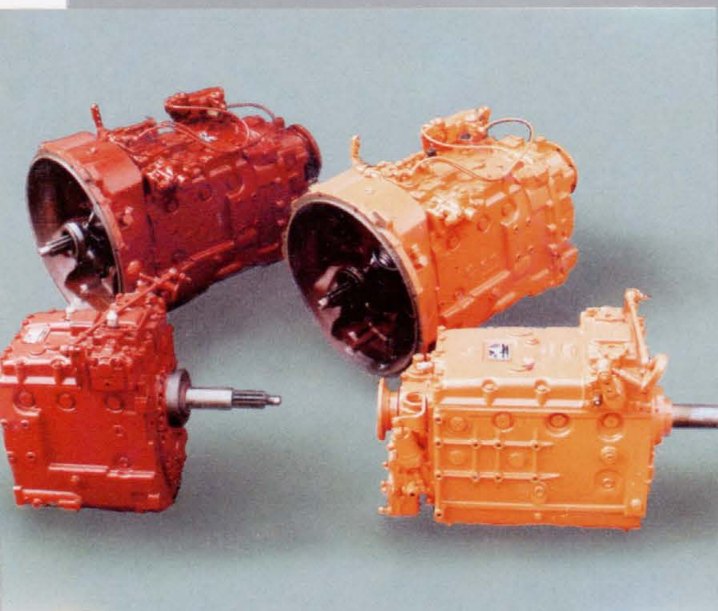
GEARBOXES, multi-speed, synchromesh for Input Torques up to 1200 Nm and corresponding POWER TAKE-OFFS. Manufacturer: FAMOS — Fabrika transmisija, Hrasnica
