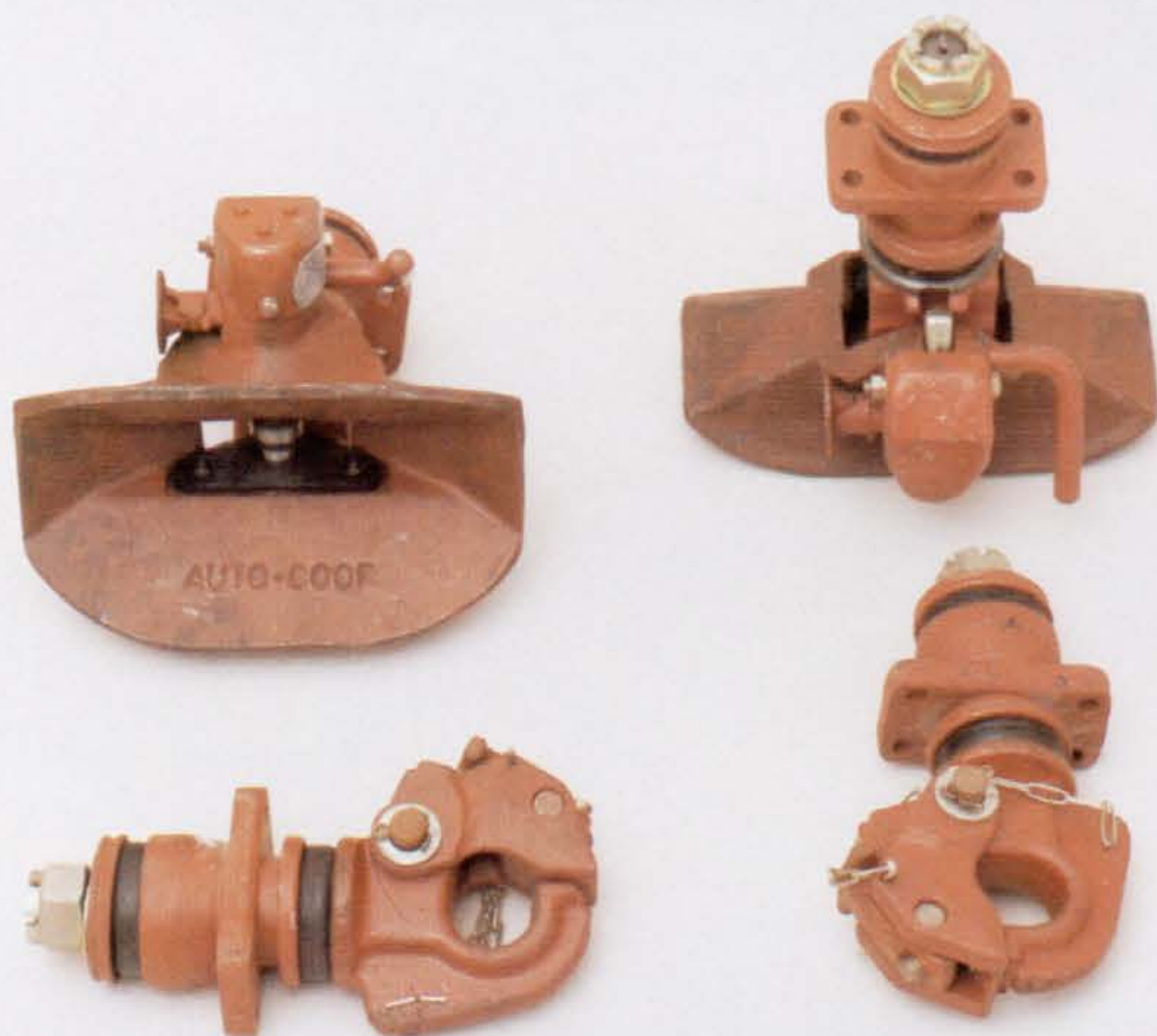
TOW HOOKS for Trucks and Cross-Country Vehicles Manufacturer: AUTO — COOP Novi Sad
