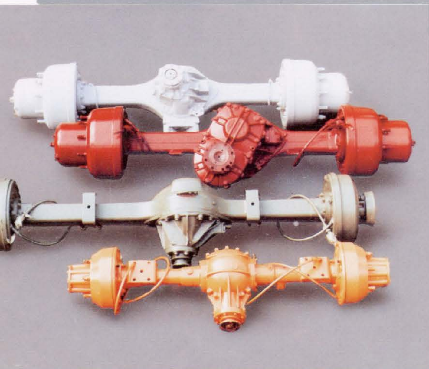
LIVE AXLES, rigid and steerable Load from 3000 to 10000 kg Manufacturer: TAM Maribor
