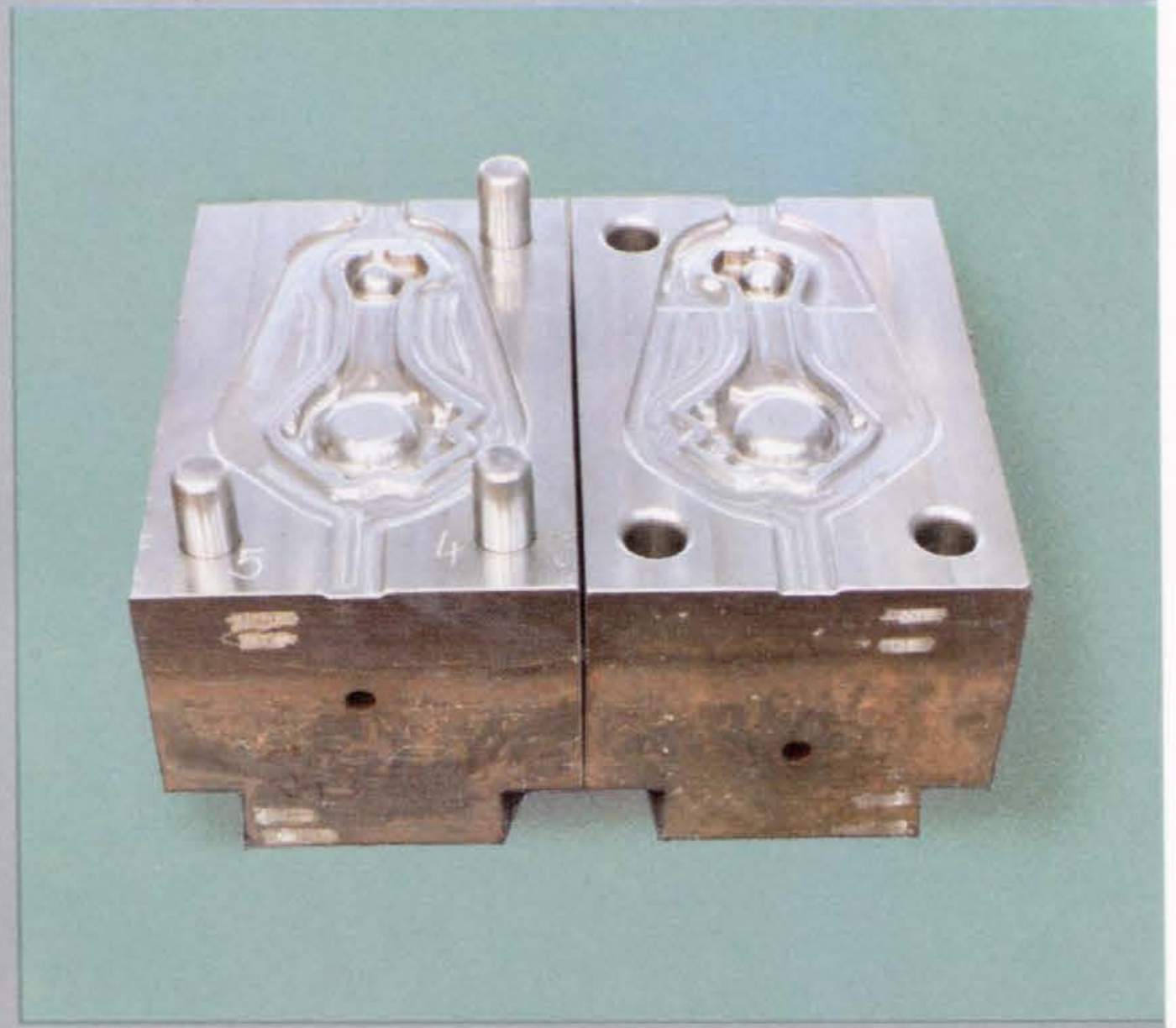
DROP-FORGE DIES Manufacturer: TAM Maribor
