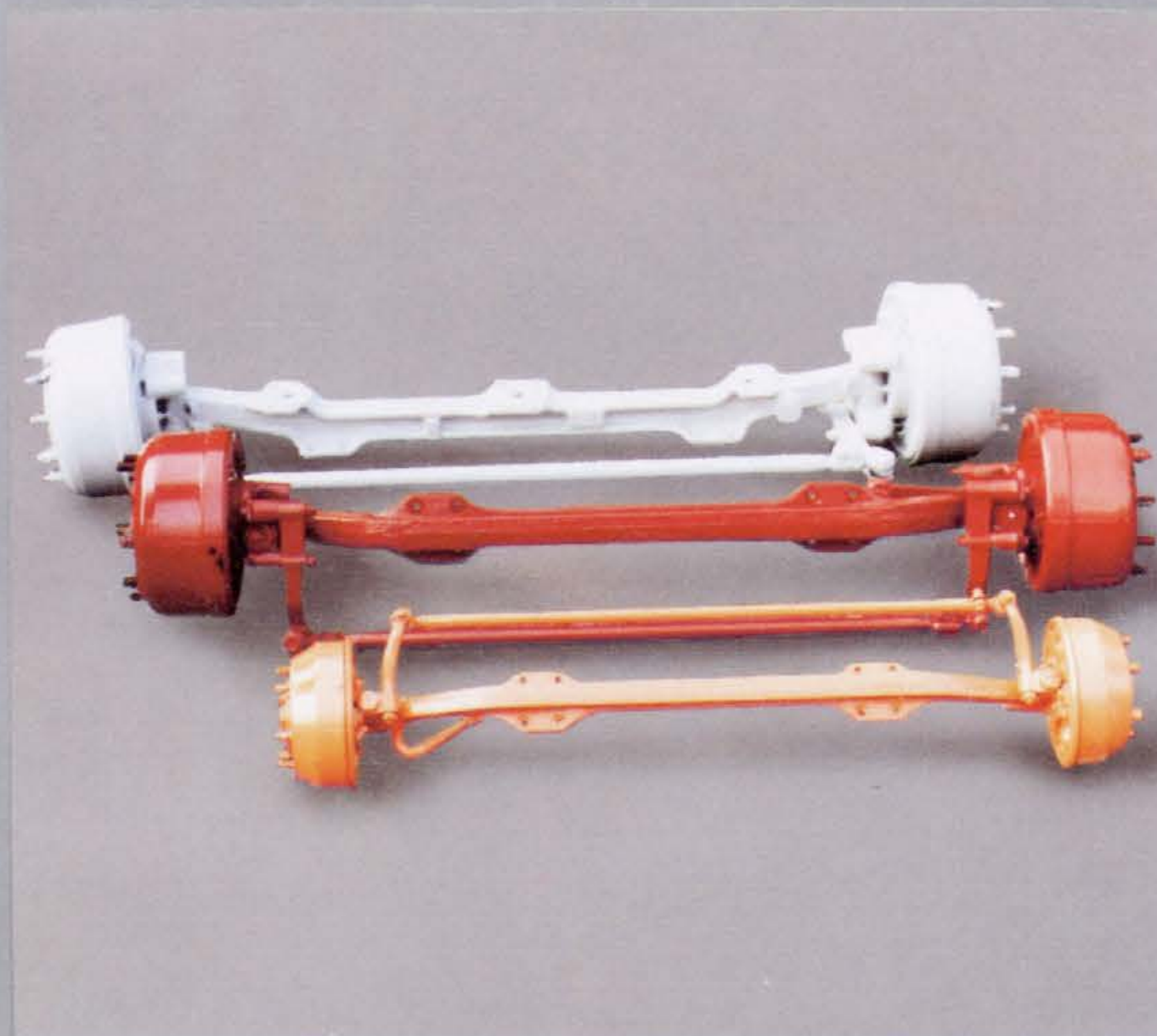
DEAD AXLES, steerable Load from 1500 to 6500 kg Manufacturer: TAM Maribor
